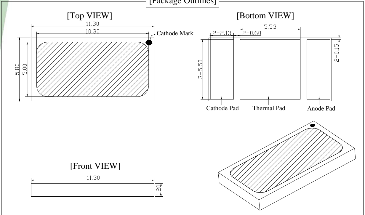
[Package Outlines]
