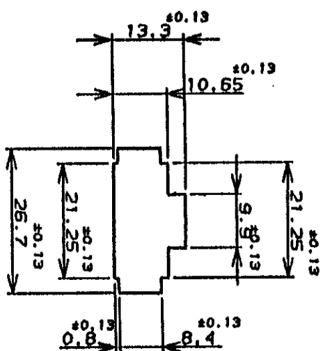
コネクタ取付寸法 (FIG. 1) RECOMMENDED PANEL OPENING DIMENSION
