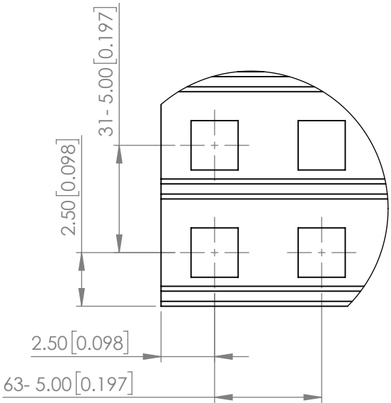
DETAIL A
