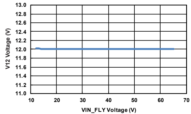
Figure 67. V12 Line Regulation, Temp = +25°C, f_{SW} = 100\text{kHz} , V6 Load = 200Ω, V12 Load = 200mA
