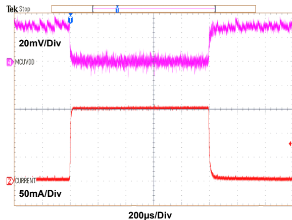
Figure 71. MCULD LDO Load Transient, I_{LOAD} = 0 to 150mA, MCULD Offset = 5.0V
