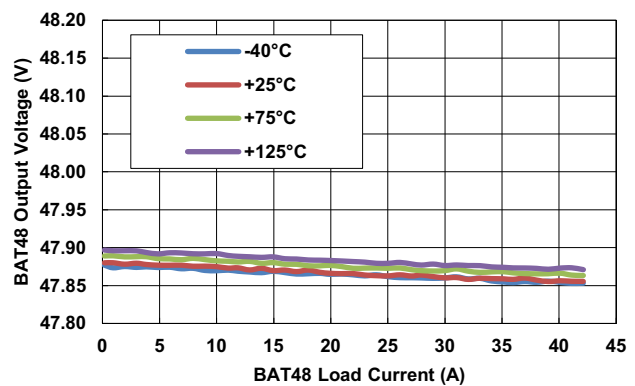
Figure 95. BAT48 Voltage In Boost/DE/NO-PD with Temperature Variable, f_{CLK} = 100\text{kHz}
