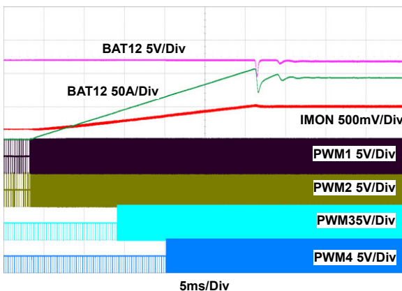
Figure 64. RL1 = 0.15\Omega \rightarrow 0.1\Omega
