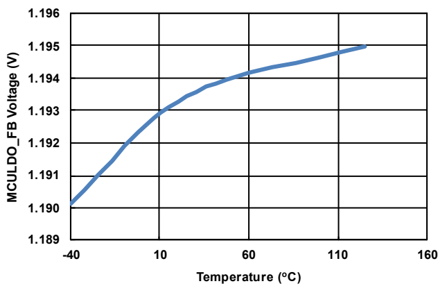
Figure 106. V_{MCU\_LDO\_FB}
