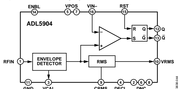
Figure 43. Functional Block Diagram
