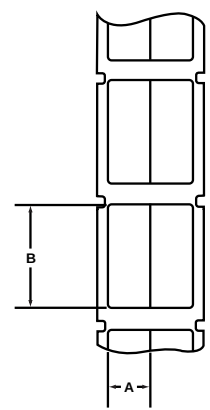
Butt-Cut
