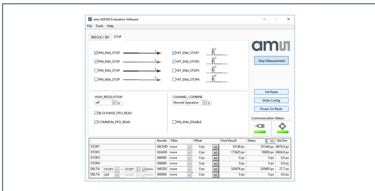
Figure 3: Setup Window
