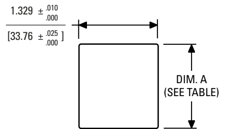
Mounting Detail
