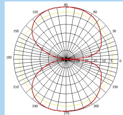
Elevation Pattern
