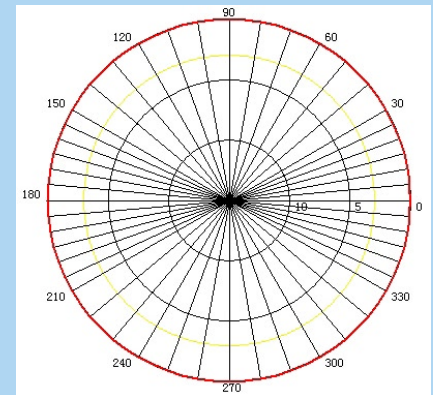
Azimuth Pattern
