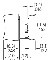
Short Actuator
