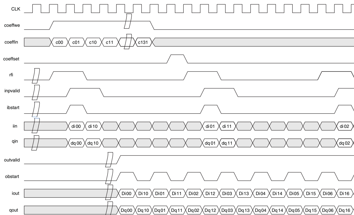
Figure 2-20. Multi-Channel (2 Channels) DHIGHSPEED I&Q Polyphase-Interpolator (1:4)
