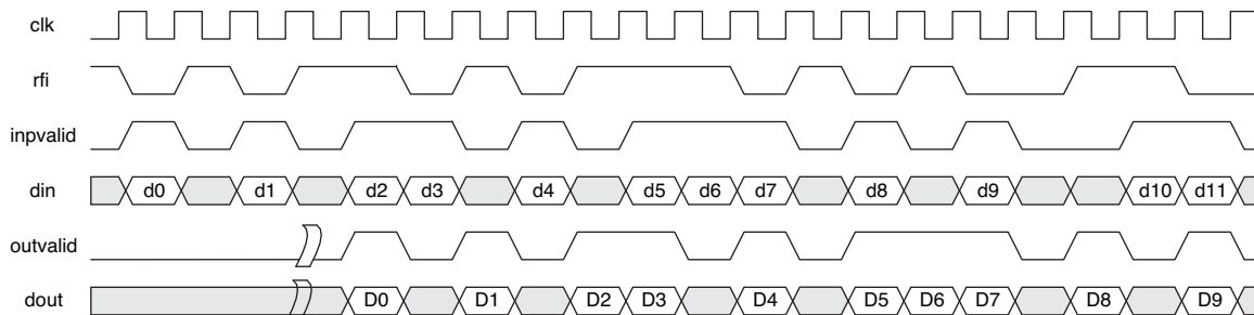
Figure 2-10. Factorset Signals
