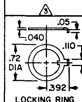
LOCKING RING
