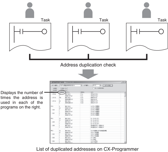
List of duplicated addresses on CX-Programmer
