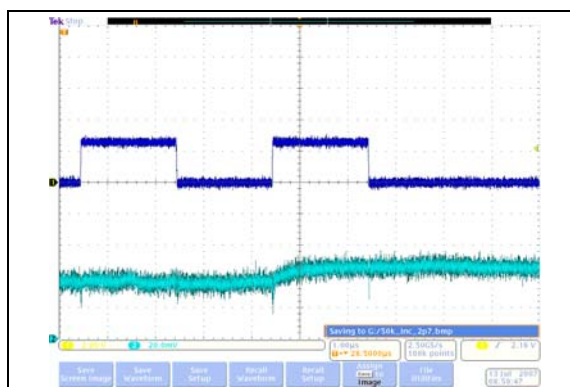
FIGURE 2-41: 50 k \Omega – Low-Voltage Increment Wiper Settling Time ( V_{DD} = 2.7\text{V} ) ( 1\text{ }\mu\text{s}/\text{Div} ).
