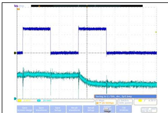
FIGURE 2-38: 50 k \Omega – Low-Voltage Decrement Wiper Settling Time ( V_{DD} = 5.5\text{V} ) ( 1\text{ }\mu\text{s}/\text{Div} ).
