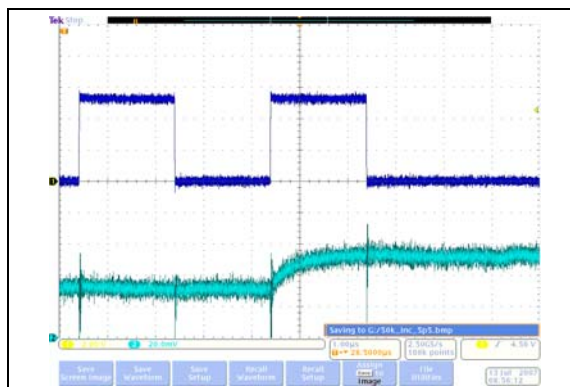
FIGURE 2-40: 50 k \Omega – Low-Voltage Increment Wiper Settling Time ( V_{DD} = 5.5\text{V} ) ( 1\text{ }\mu\text{s}/\text{Div} ).
