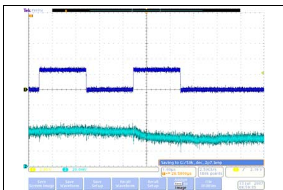
FIGURE 2-39: 50 k \Omega – Low-Voltage Decrement Wiper Settling Time ( V_{DD} = 2.7\text{V} ) ( 1\text{ }\mu\text{s}/\text{Div} ).
