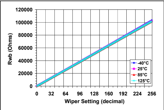
FIGURE 2-49: 100 kΩ – R_{WB} ( \Omega ) vs. Wiper Setting and Ambient Temperature.
