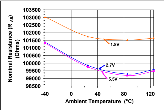
FIGURE 2-48: 100 kΩ – Nominal Resistance ( \Omega ) vs. Ambient Temperature and V_{DD} .
