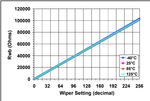
FIGURE 2-49: 100 k\Omega – R_{WB} ( \Omega ) vs. Wiper Setting and Ambient Temperature.
