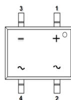
Pin Diagram
