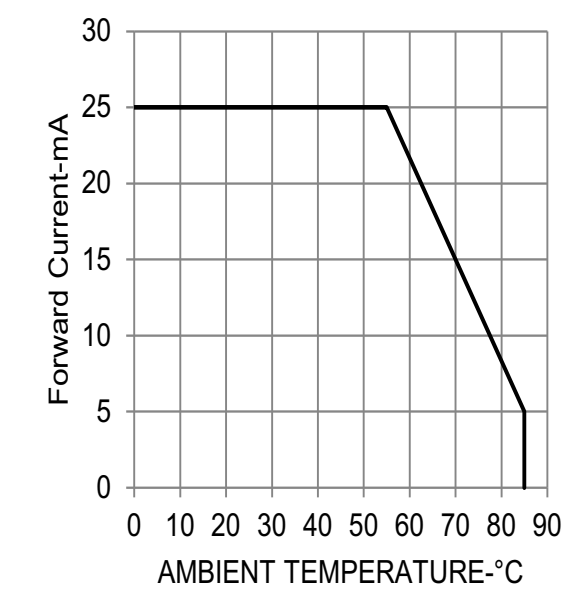
Figure 10: Derating Curve
