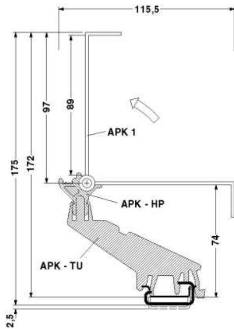
Dimensioned drawing
