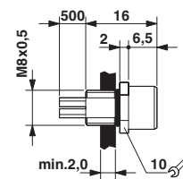
M8 flush-type socket
