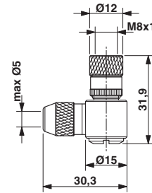
Socket M8 x 1, angled, shielded
