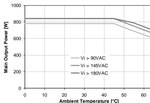
Figure 42. Thermal derating for PFE850-12-054RA
