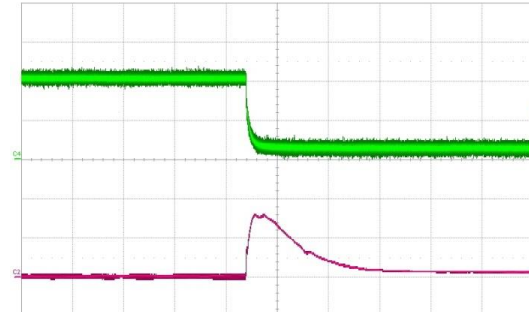
Figure 16. Load transient V 1 , 40 to 5 A (500 μs/div) CH2: V 1 (200 mV/div) CH4: I 1 (20 A/div)
