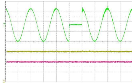
Figure 12. AC drop out 10 ms (10ms/div) CH1: V 1 (2V/div) CH2: V SB (1V/div) CH4: V n (200V/div)
