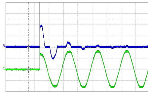
Figure 5. Inrush current, V_{in} = 230\text{Vac} , 90^\circ CH4: V_{in} (200V/div), CH2: I_{in} (20 A/div)
