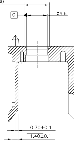
SECTION B-B
