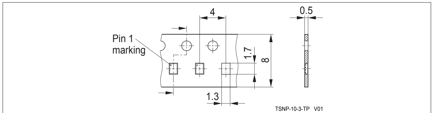
Figure 13: TSNP-10-3 Carrier Tape
