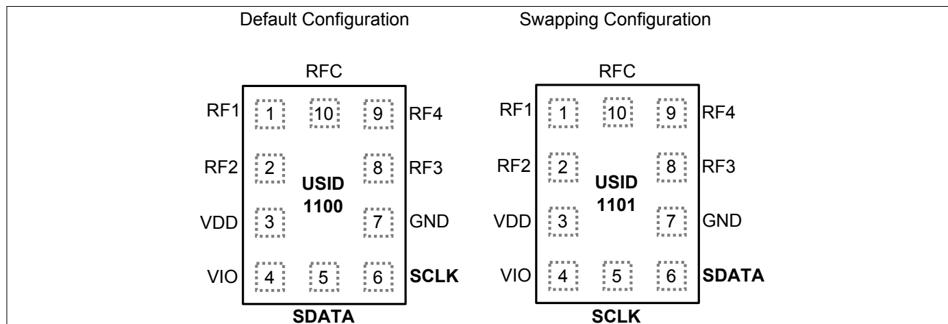
Figure 9: BGSA141MN10 Pin Configuration - USID 1100 and USID 1101 (top view)
