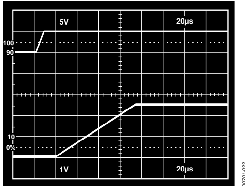
Figure 22. Turn-On Characteristics
