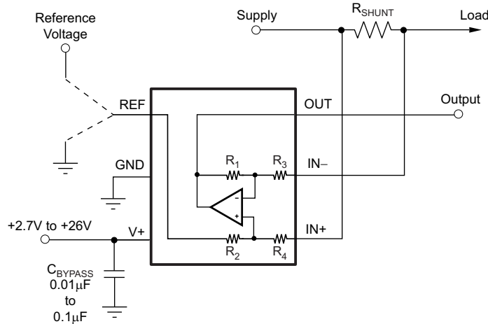
Figure 20. Typical Application
