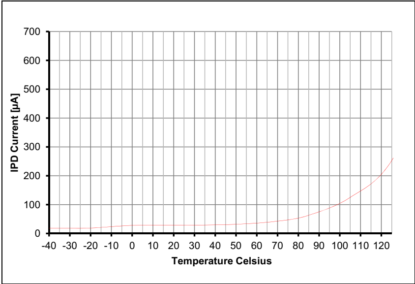
FIGURE 26-9: TYPICAL I PD CURRENT @ V DD = 3.3V, +85°C
