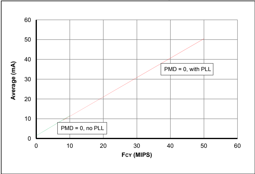
FIGURE 26-10: TYPICAL I DD CURRENT @ V DD = 3.3V, +85°C
