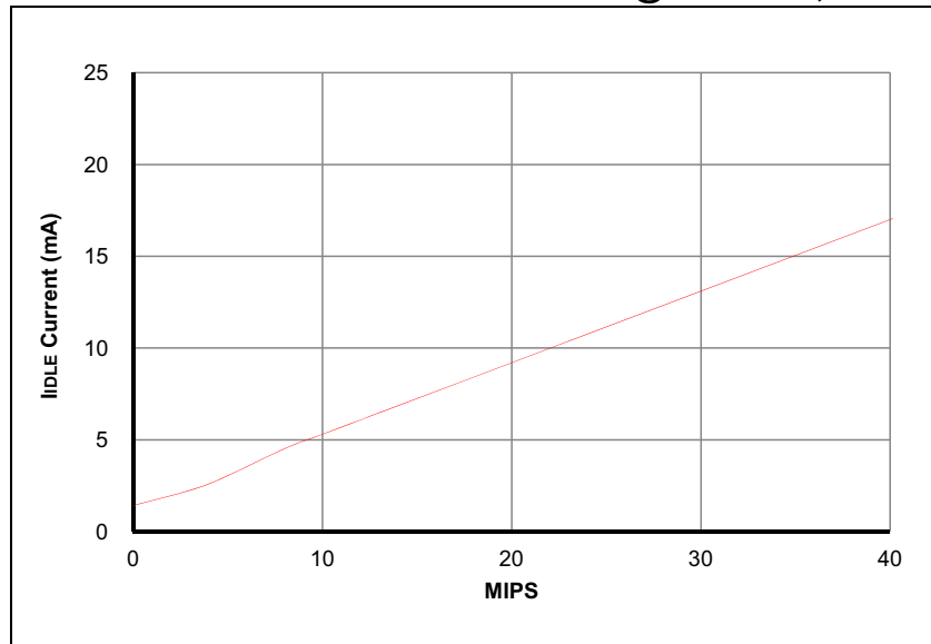
FIGURE 26-12: TYPICAL I IDLE CURRENT @ V DD = 3.3V, +85°C
