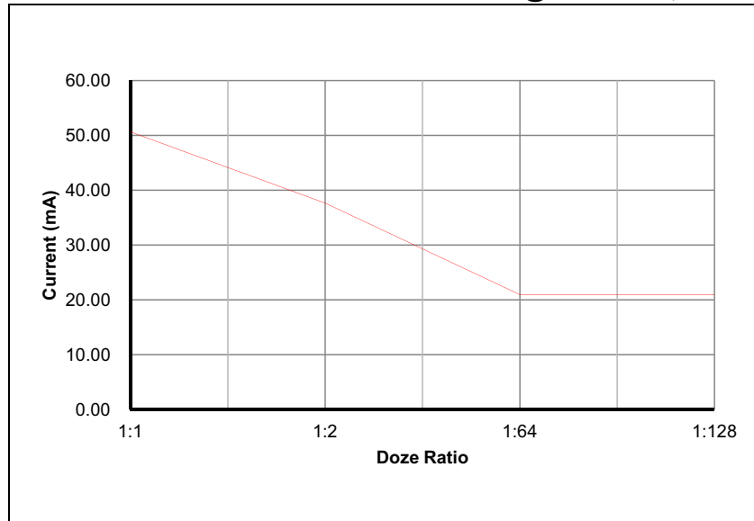
FIGURE 26-11: TYPICAL I DOZE CURRENT @ V DD = 3.3V, +85°C
