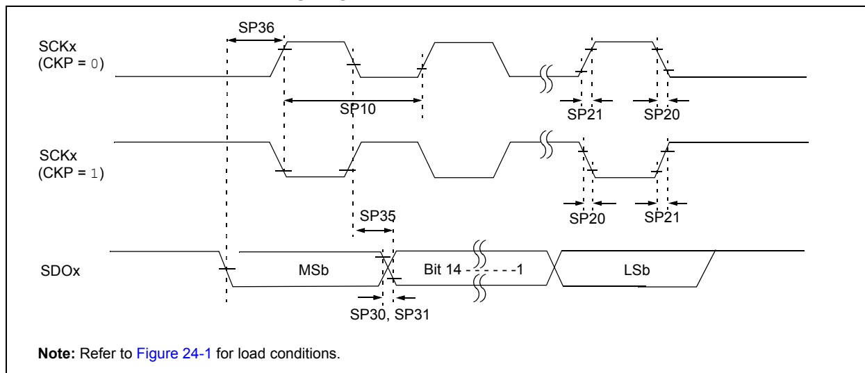
FIGURE 24-15: SPIx MASTER MODE (HALF-DUPLEX, TRANSMIT ONLY) CKP = 1) TIMING CHARACTERISTICS
