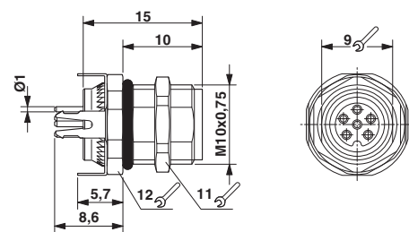
M8 flush-type socket
