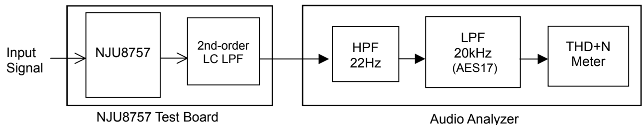
Figure 1. Output THD+N
