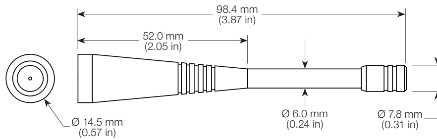
Figure6. CW LTE Band 28 Antenna Dimensions
