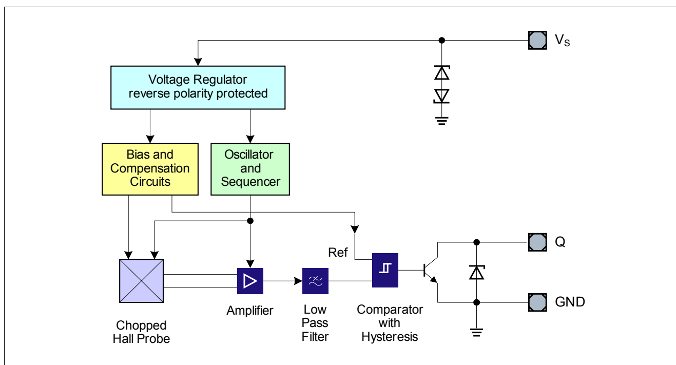
Figure 2 TLV4906K Block Diagram
