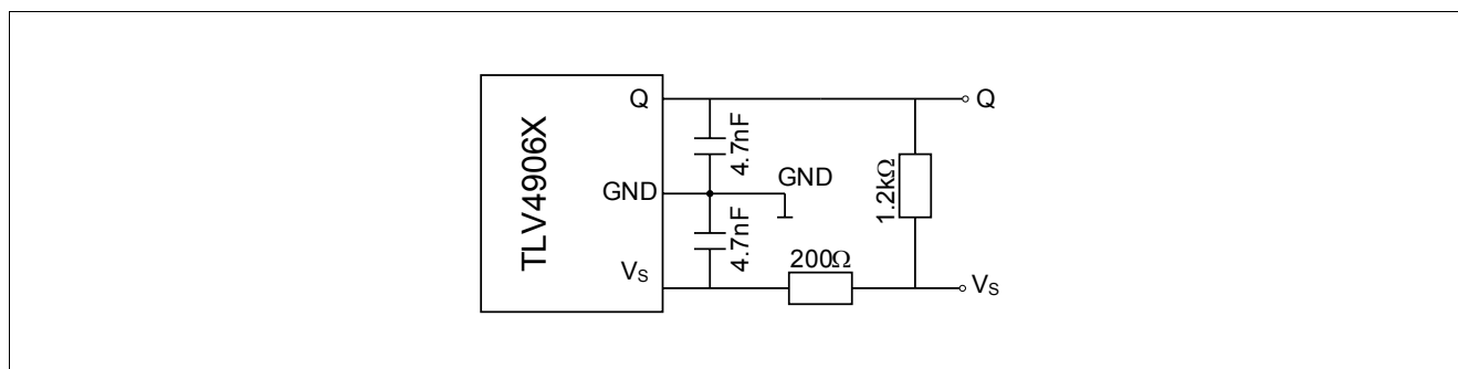
Figure 5 Application circuit
