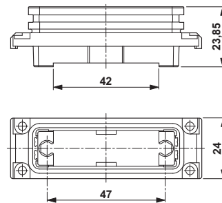
Adapter plate
