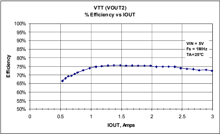
Figure 5. % Efficiency vs. IOU
