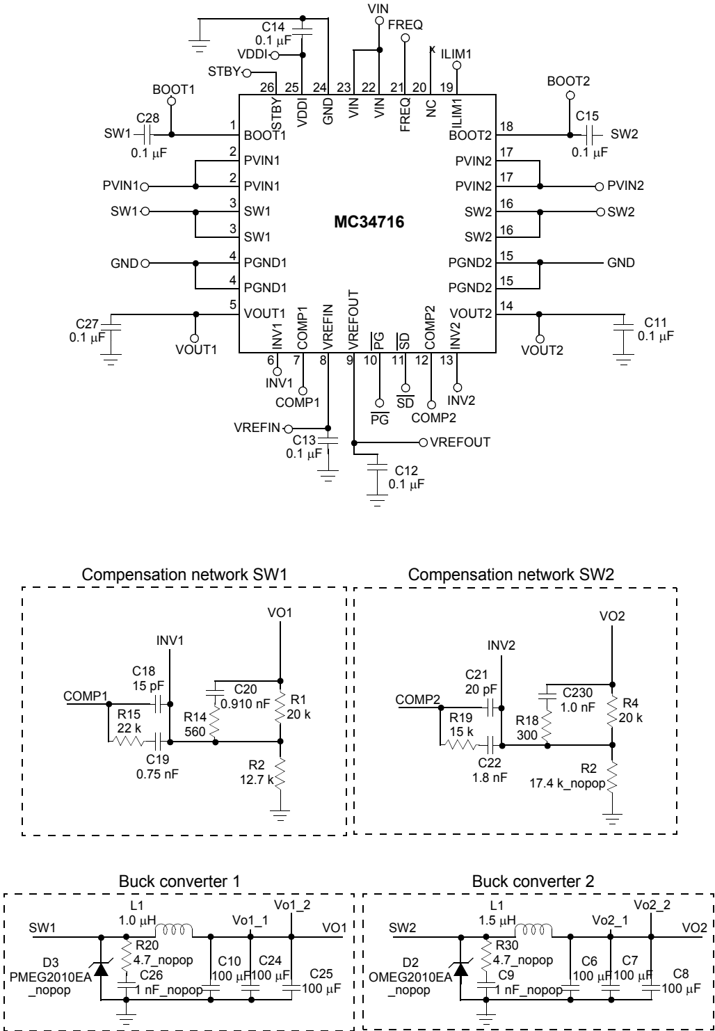
Figure 9. Typical application
