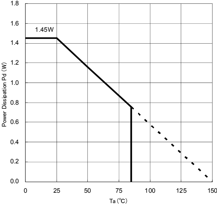
Fig. 9 Power dissipation
