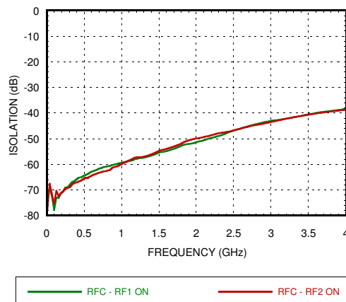
Isolation Between Ports RF1 and RF2
