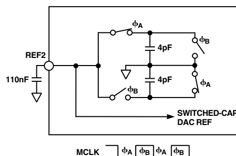
Figure 10. REF2 Equivalent Circuit
