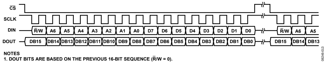
Figure 11. SPI Communication Bit Sequence
