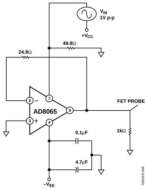
Figure 48. Positive PSRR
