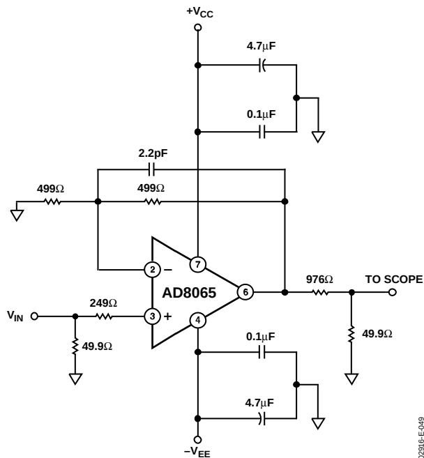
Figure 49. Settling Time
