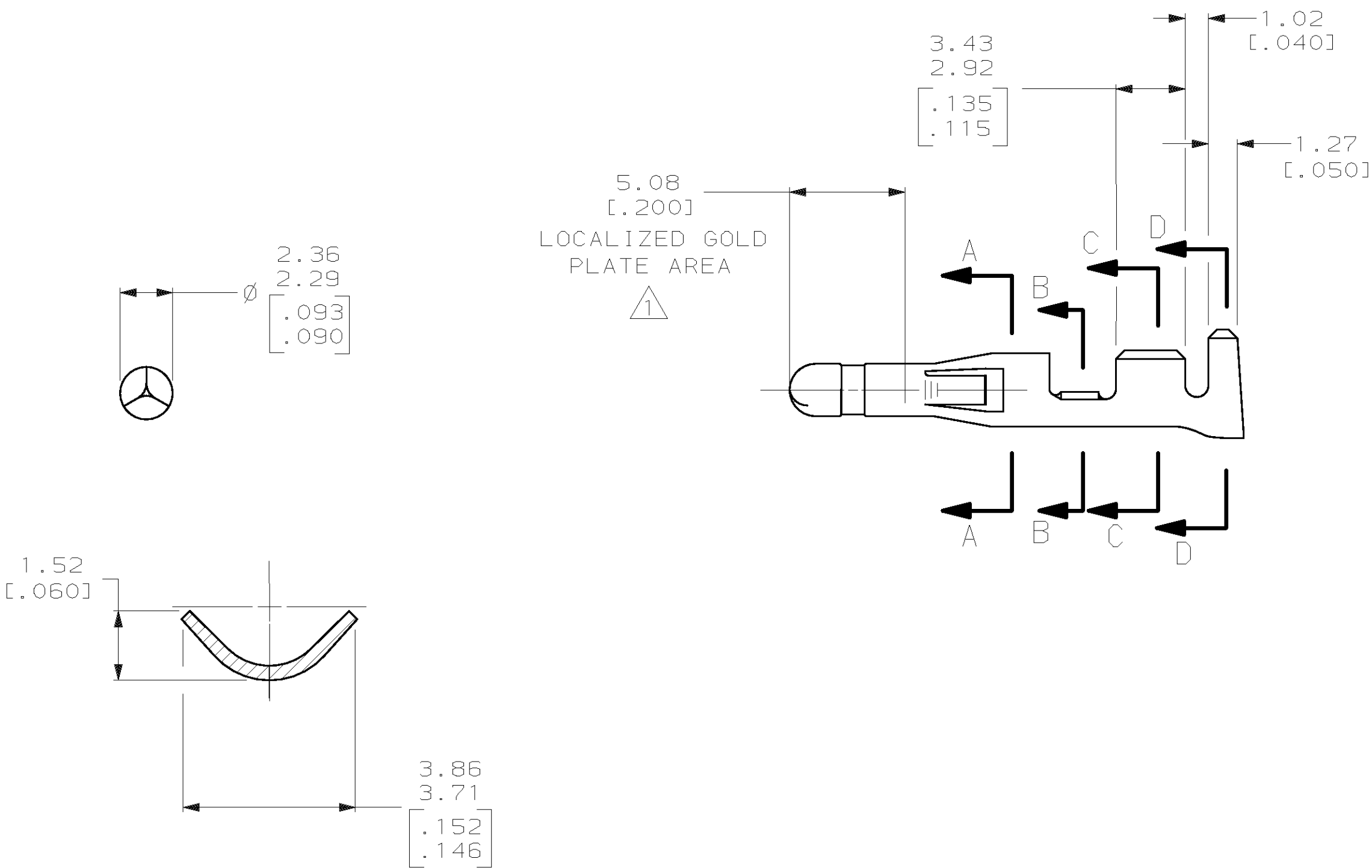
SECTION B-B SCALE 10:1
