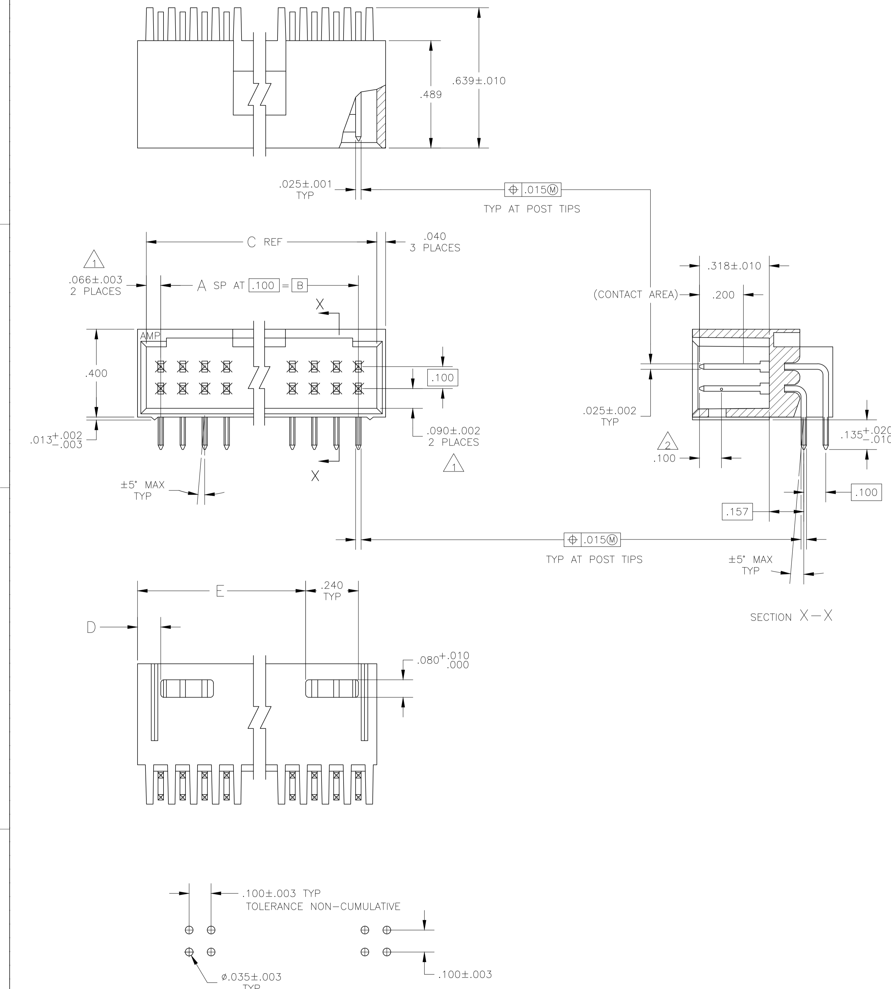
RECOMMENDED HOLE LAYOUT
