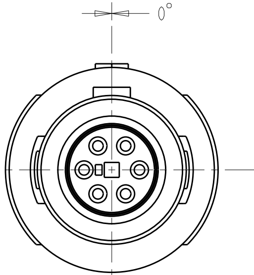
0° KEYING SCALE 4:1
