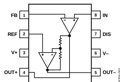
Figure 1. SOIC/LSCSP Pinout
