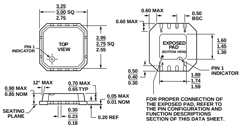
Figure 59. 8-Lead Lead Frame Chip Scale Package [LFCSP_VD] 3 mm × 3 mm Body, Very Thin, Dual Lead (CP-8-2)
