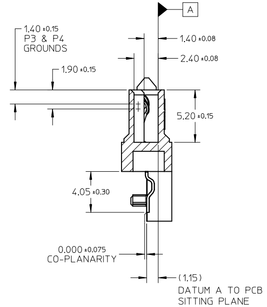
SECTION Z-Z
