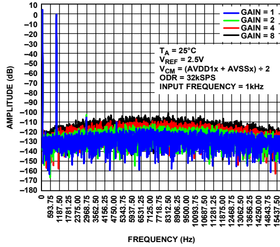
Figure 41. FFT Plot, Low Power Mode at 32 kSPS, Input Frequency ( f_{IN} ) = 1 kHz, Sinc5 Filter Enabled
