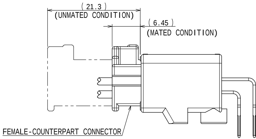
MATING CONDITION(REF.)
