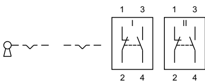
73 Keylock switch 2 positions page 9 | Keylock switch actuator 2 positions, flush mounting page 15
