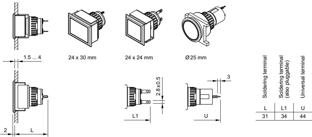
16 Illuminated pushbutton actuator, flush mounting page 14
